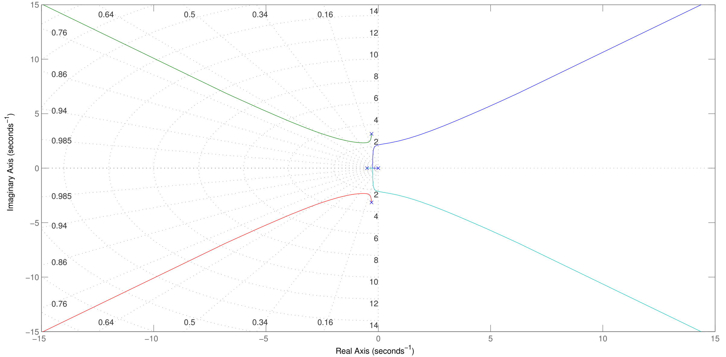
Root Locus
